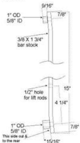
LOWER LIFT ARMS (2) (Last 1 1/2" - 2" of each end bent 5deg)
